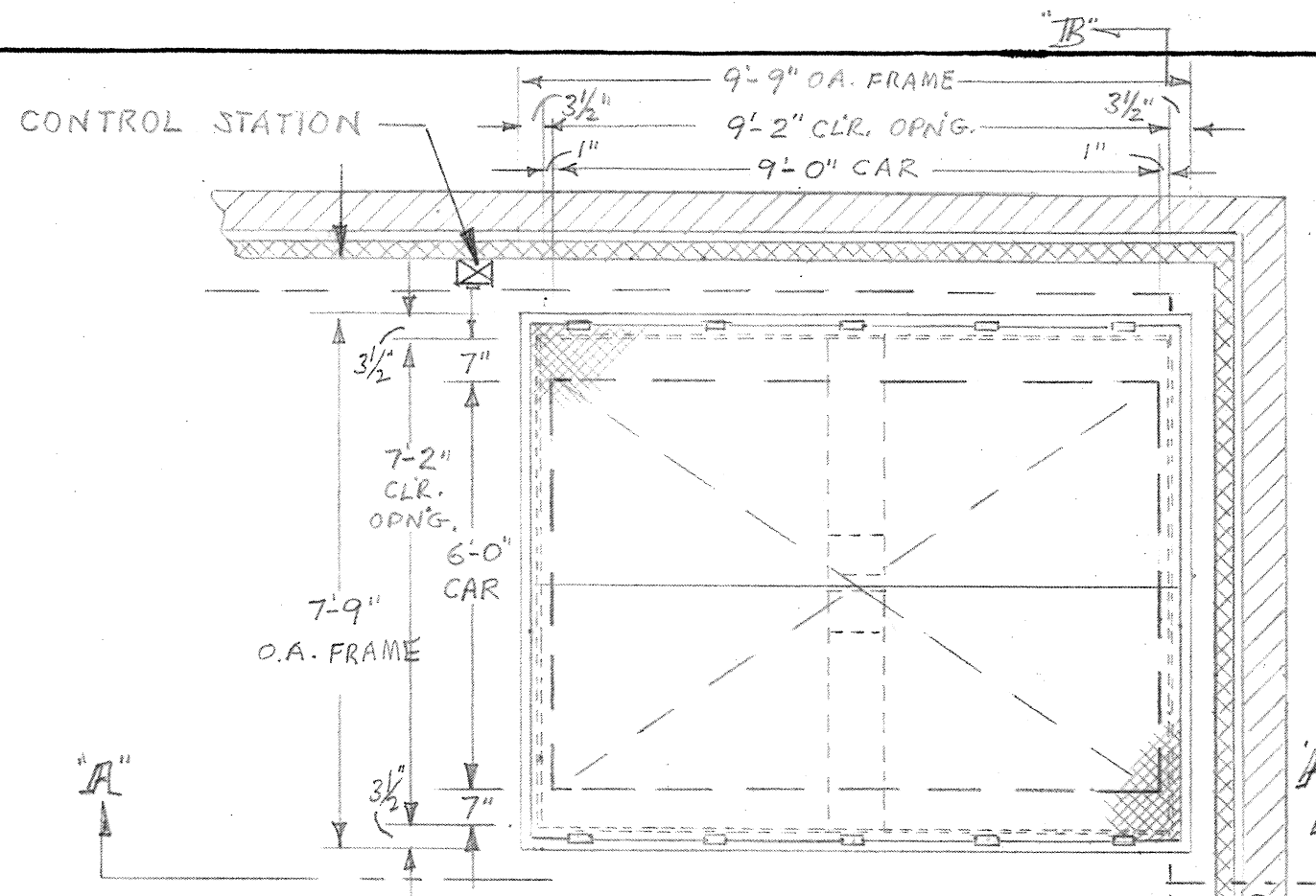
VIEW UPPER LEVEL
