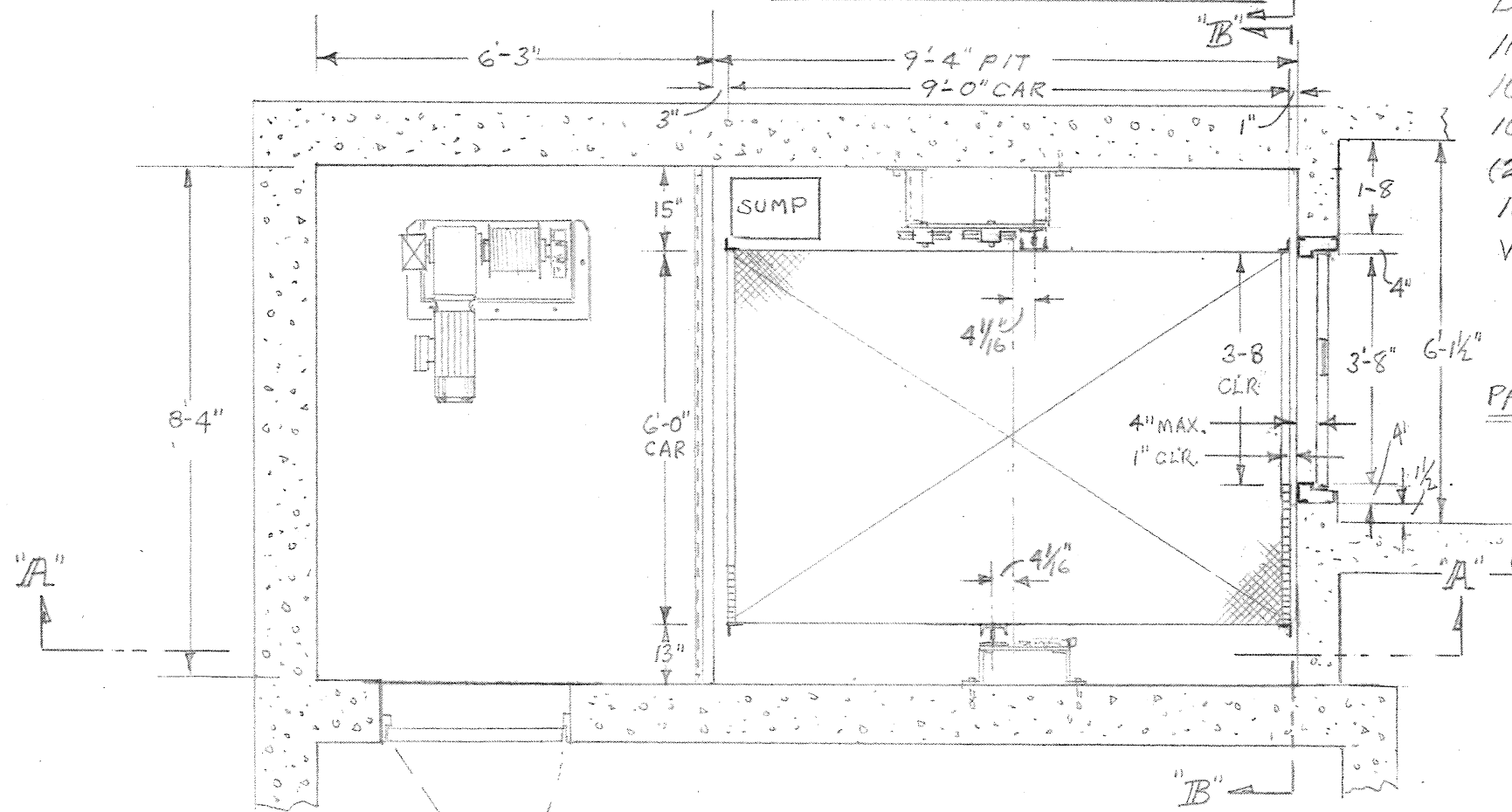
VIEW LOWER LEVEL
